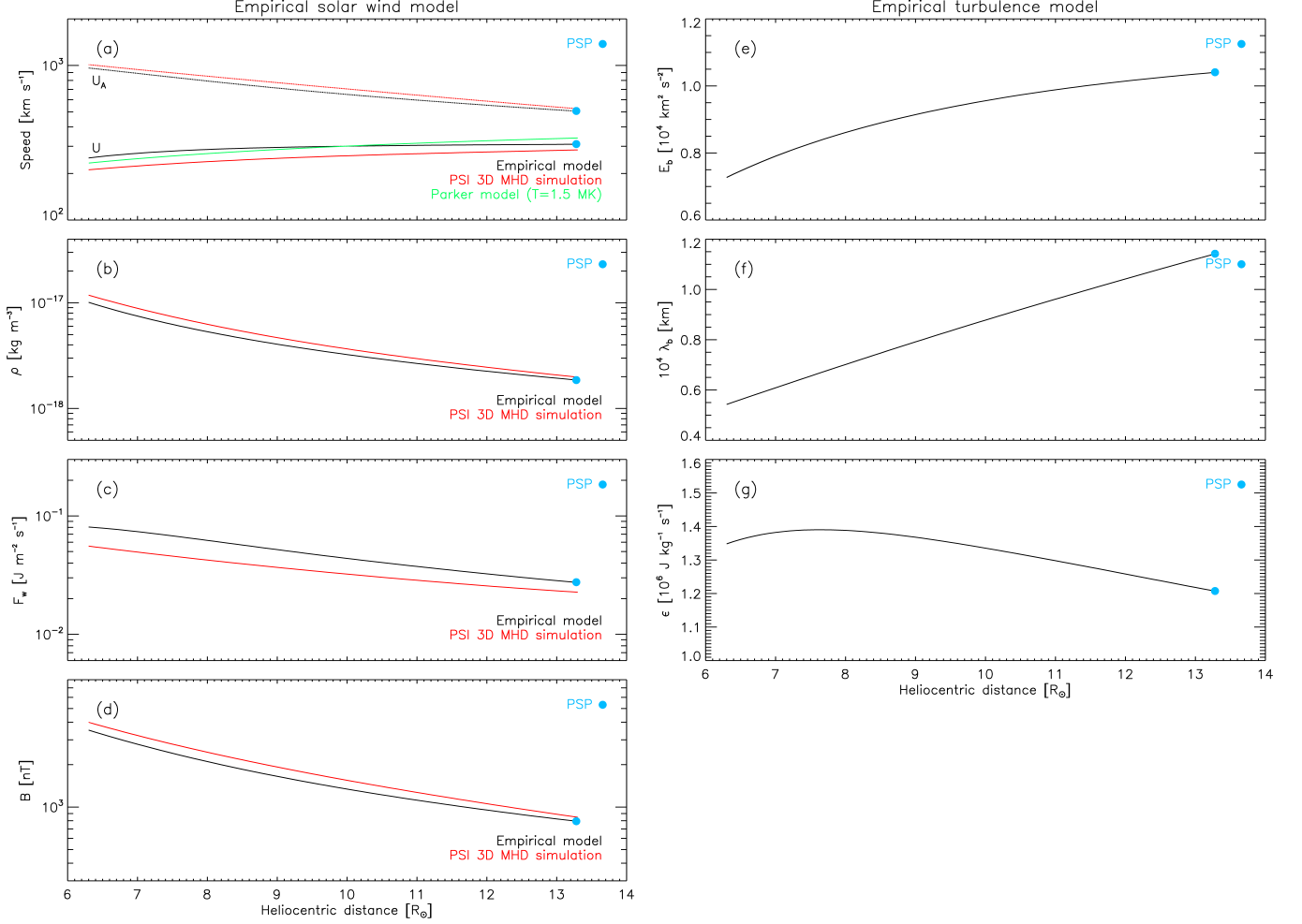
Figure 2. Data-based (black) and physics-based (red) modeling of the radial evolution of solar wind U (thick lines) and Alfvén U_A (thin lines) speed (a), plasma mass density \rho (b), solar wind flux energy F_w (c), magnetic field B (d), turbulent energy E_t (e) and correlation length \lambda_b (f), and heating rate \epsilon (g) in the slow coronal flow jointly observed with SO/Metis and PSP during their quadrature on June 01, 2022. The blue dot in each panel refers to the values obtained with PSP measurements. The Parker classical model for an expanding isothermal 1.5 MK corona is shown as a green line in (a).
