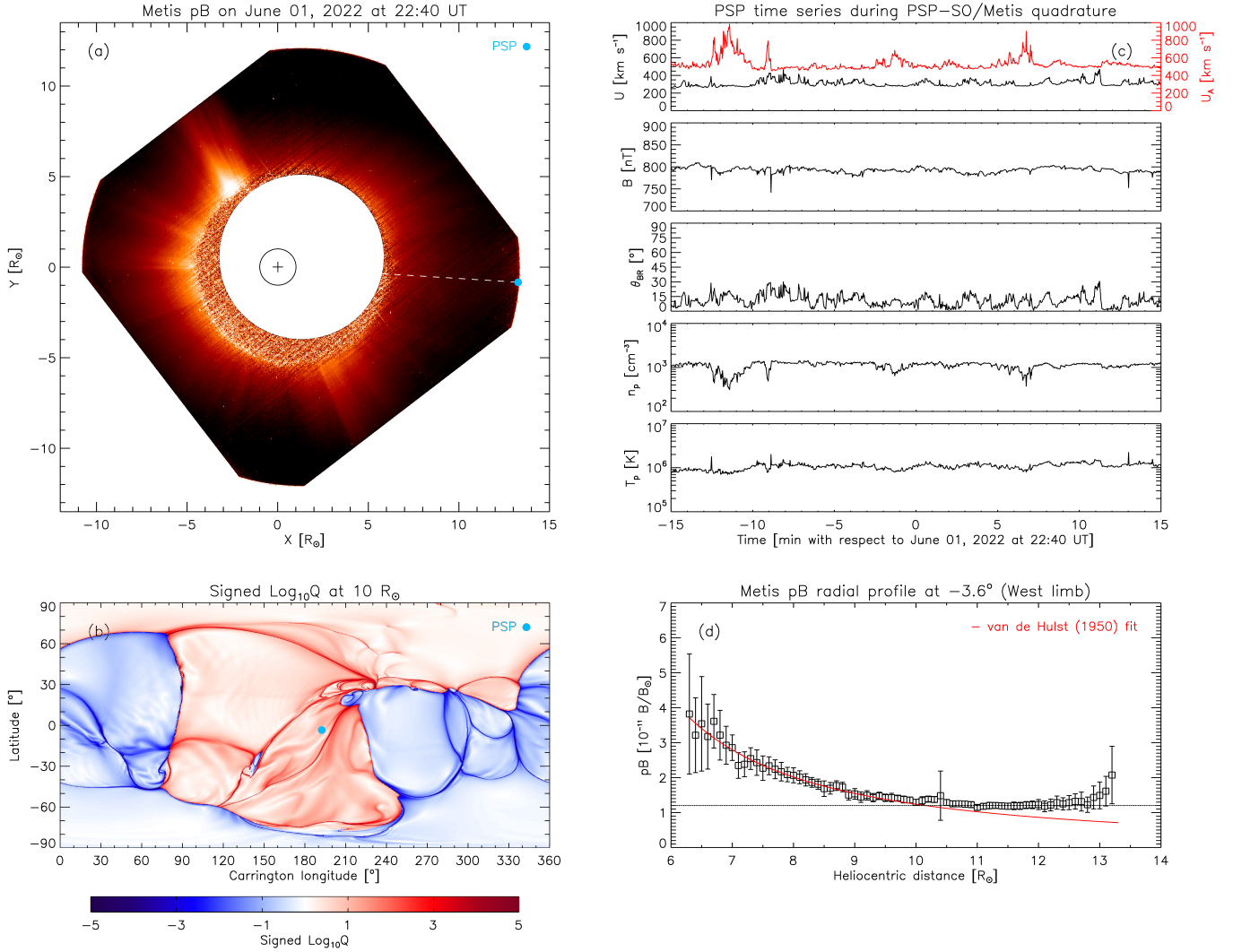
Figure 1. (a) Metis pB image on June 01, 2022 at 22:40 UT with PSP marked in its POS as a blue dot; the PSP direction is indicated by a white dashed line. (b) Projection of the PSP position (blue dot) onto the Carrington map of the squashing factor Q at 10 R_{\odot} . (c) PSP magnetic field and plasma time series (from top to bottom: wind bulk and Alfvén speed, magnetic field intensity and angle with the radial, proton density and temperature) during the quadrature with SO. (d) Radial profile of the Metis pB observations at the latitude corresponding to the PSP location (open squares), along with the van de Hulst (1950) power-law fit (red line); the horizontal line at 1.2 \times 10^{-11} B/B_{\odot} represents the flattening level probably due to the contamination by the F corona and instrumental effect.
